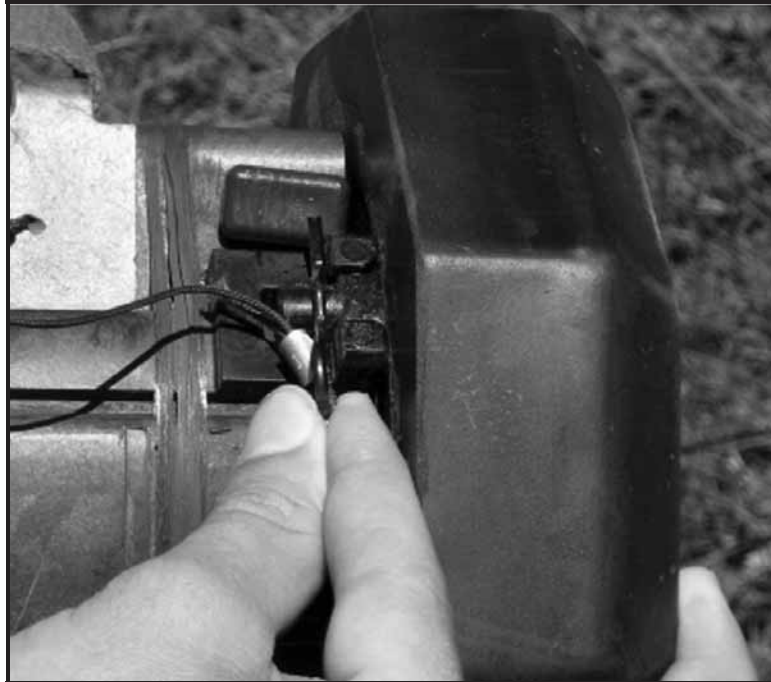
Figure 3-15. Removing the transport safety pin on the M141 bunker defeat munition.
