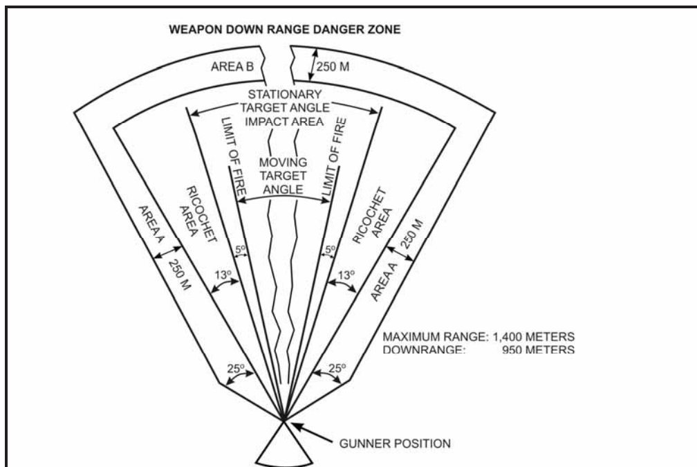
Figure 2-16. Downrange danger area for the M72A4/A5/A6/A7.
