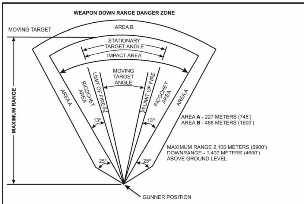
Figure 2-15. Downrange danger area for the M136A1 AT4 confined space.
