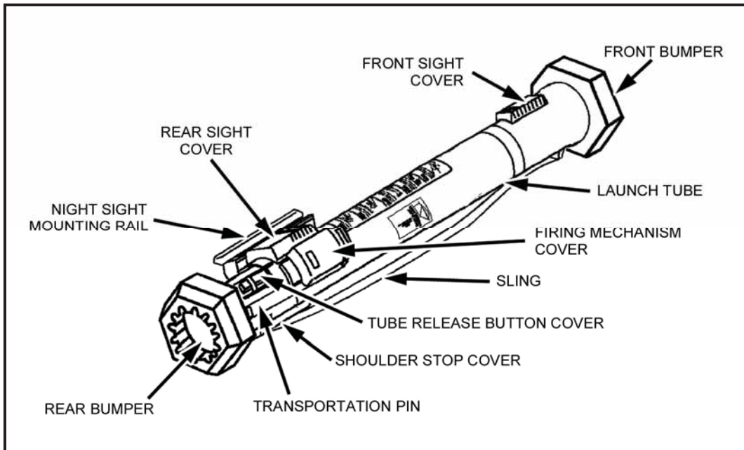
Figure 3-2. M141 bunker defeat munition inspection points.
