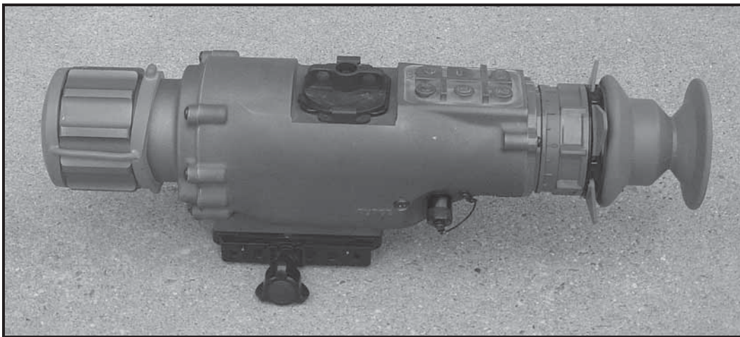
Figure C-5. AN/PAS-13E light weapon thermal sight.
